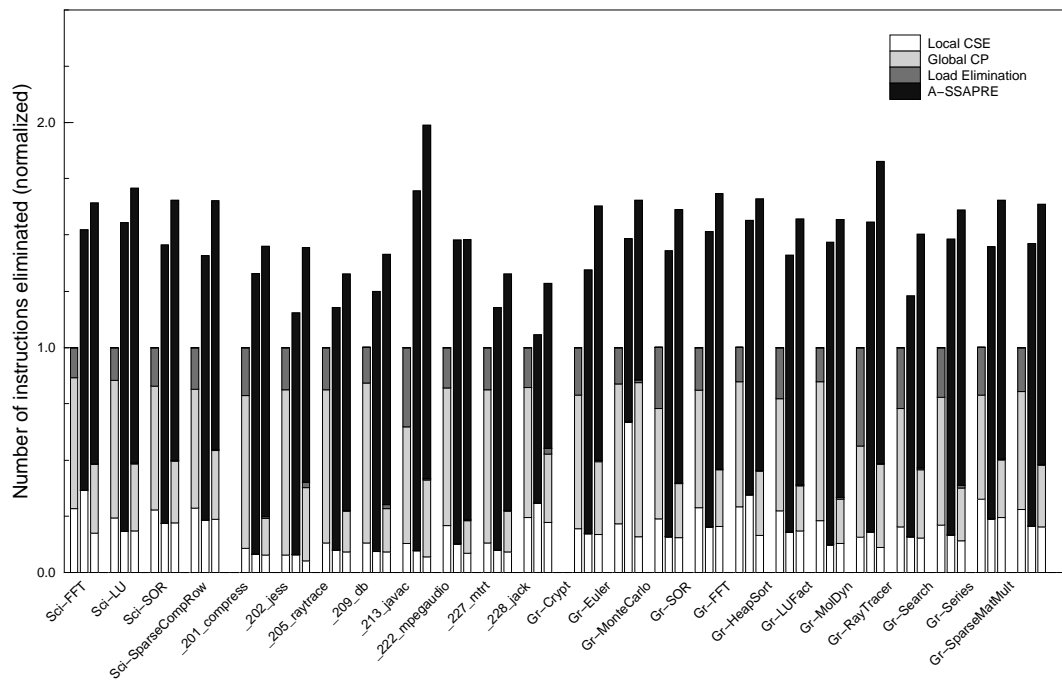
Figure 13. Static results for the benchmarks
