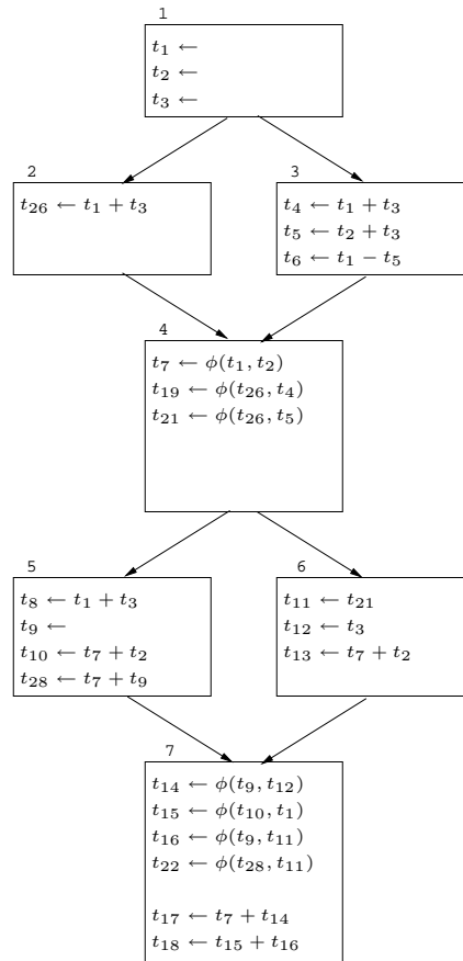
Figure 12. Optimized
