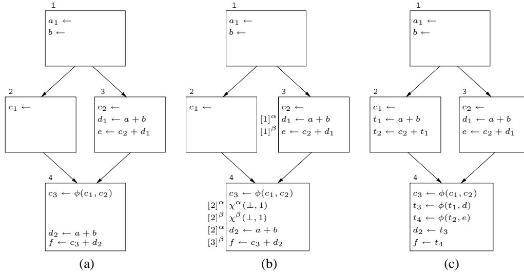
Figure 7. Nested redundancy
