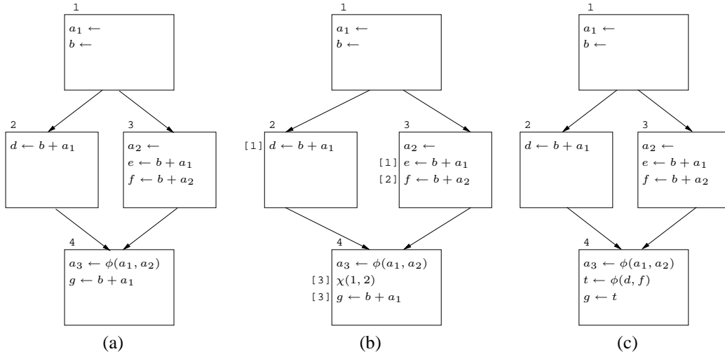
Figure 4. PRE example 1 after constant copy propagation
