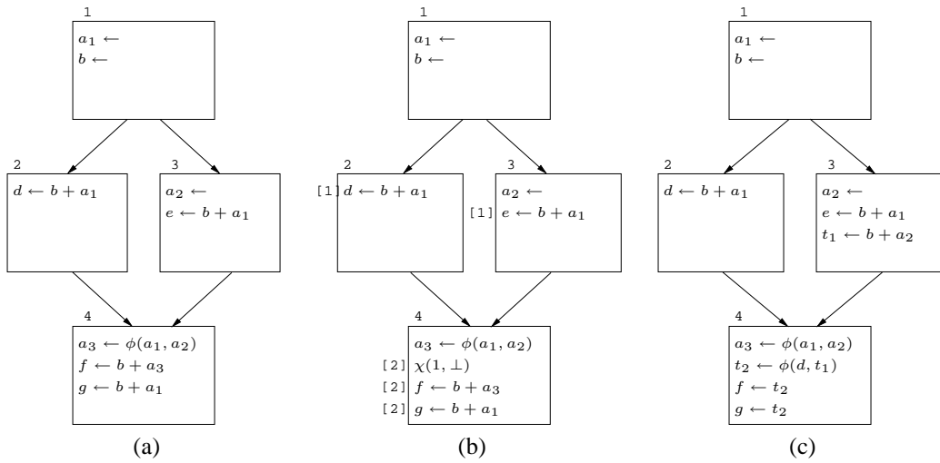
Figure 6. PRE example 2 after Constant Copy Propagation
