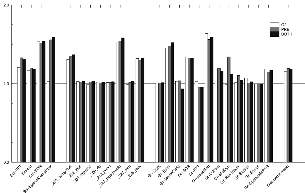
Figure 14. Speedup on benchmarks
