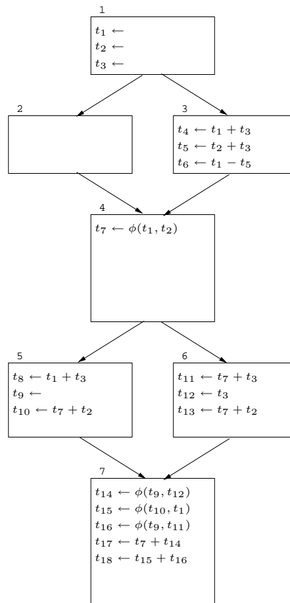
Figure 9. Unoptimized
