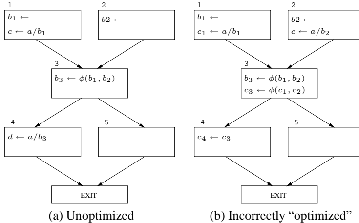
Figure 2. Illicit code motion
