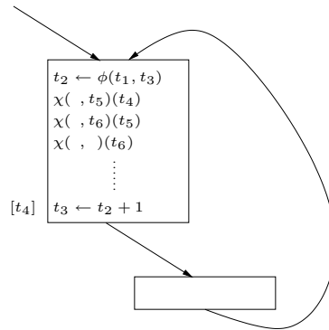
Figure 11. Unterminated \chi insertion
