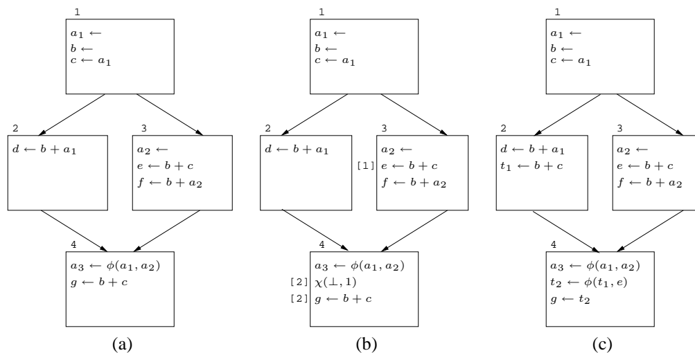
Figure 3. PRE example 1
