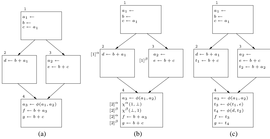
Figure 5. PRE example 2
