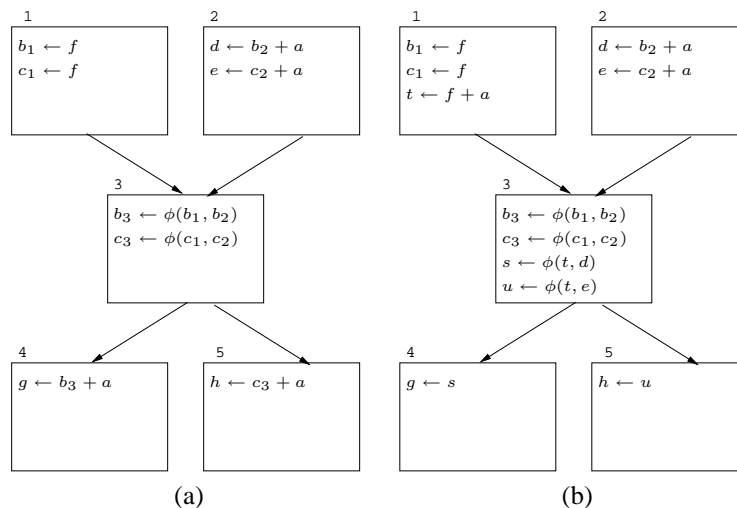
Figure 8. Redundancy eliminated by Bodík et al.
