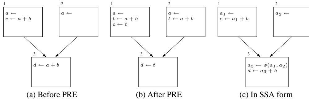
Figure 1. Basic example
