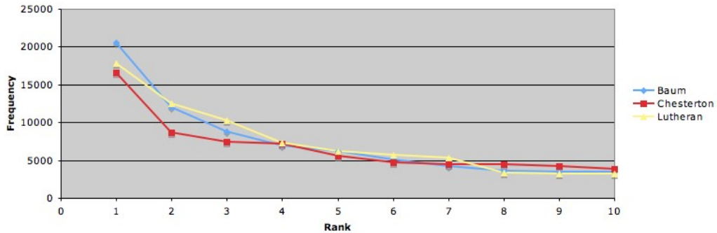
Rank vs frequency, close-up
