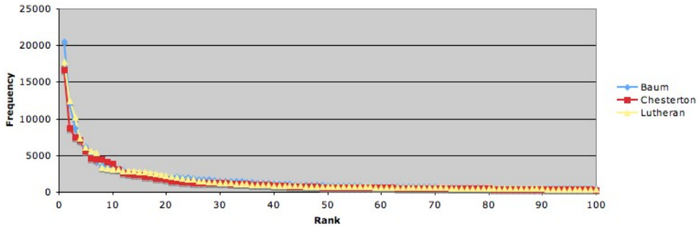
Rank vs frequency
