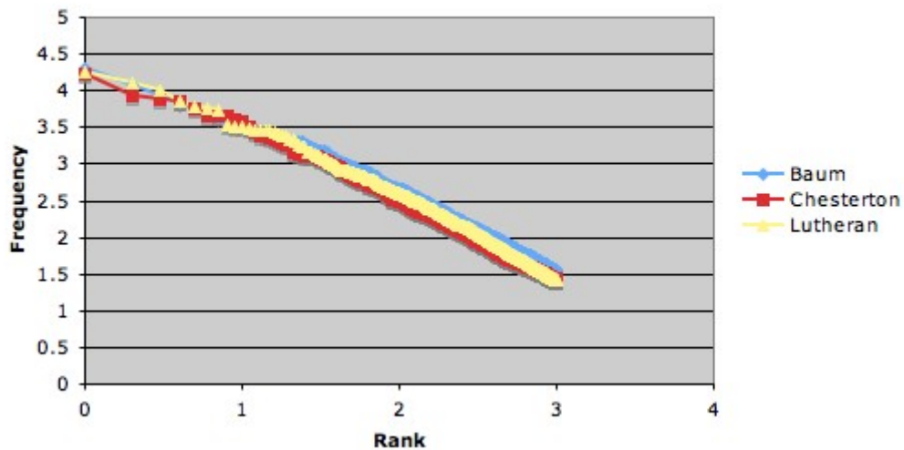
Rank vs frequency, log-log
