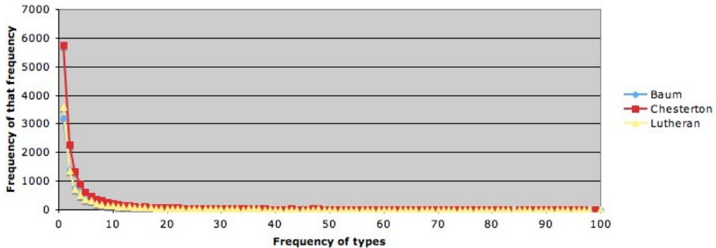
Frequency of the frequencies
