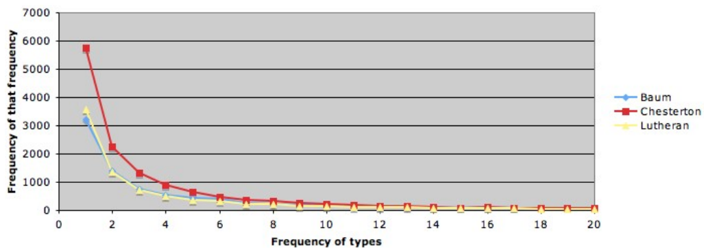
Frequency of the frequencies
