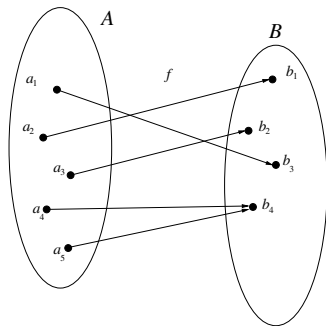
Onto but not one-to-one
