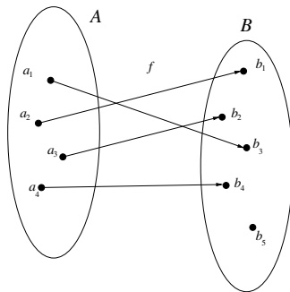
One-to-one but not onto
